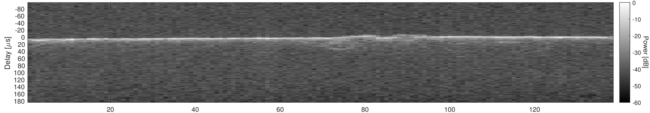
Orbit 13106, Cluttergram
