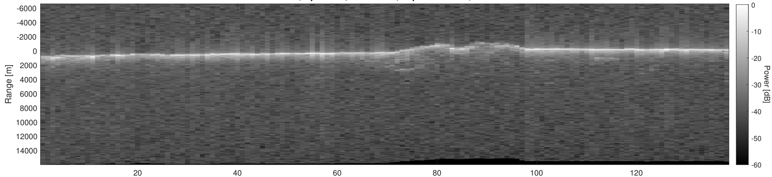
Orbit 13106, Depth-Corrected Cluttergram
