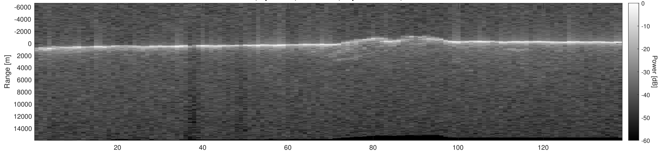
Orbit 13106, Optimized, No Window, Depth-Corrected, Channel 2
