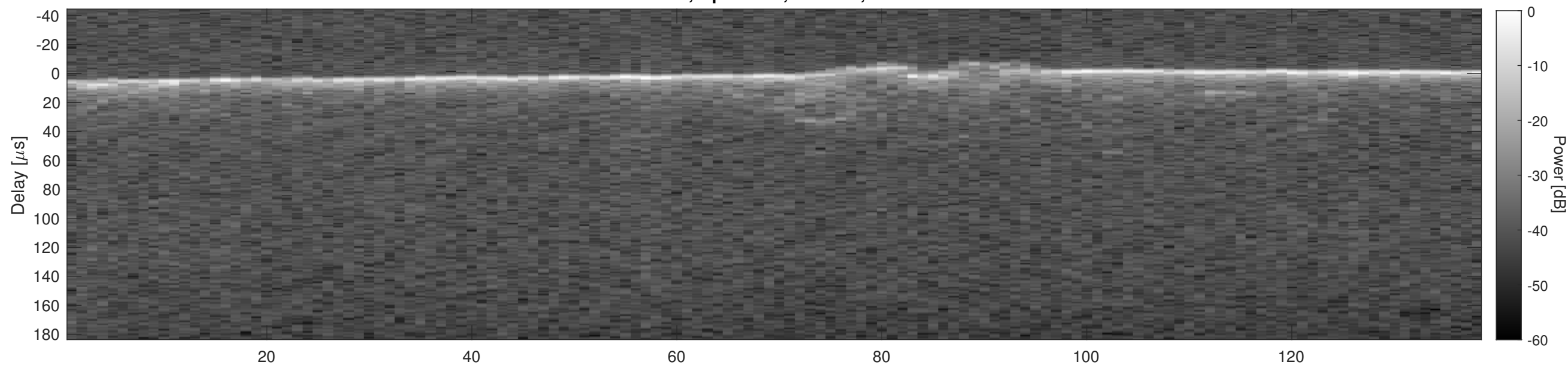
Orbit 13106, Cluttergram
