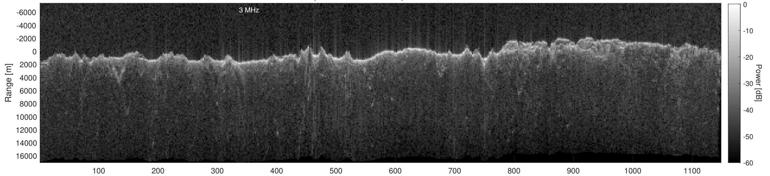
Orbit 13121, Depth-Corrected Cluttergram
