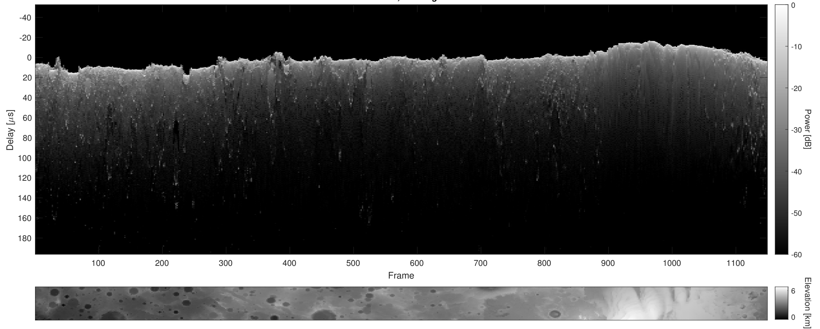
Orbit 13122, Cluttergram
