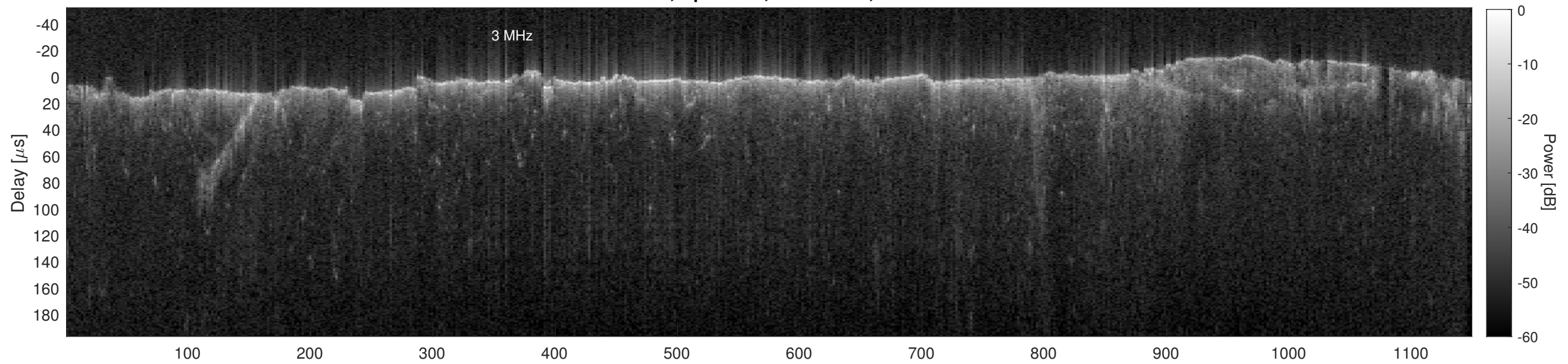
Orbit 13122, Cluttergram
