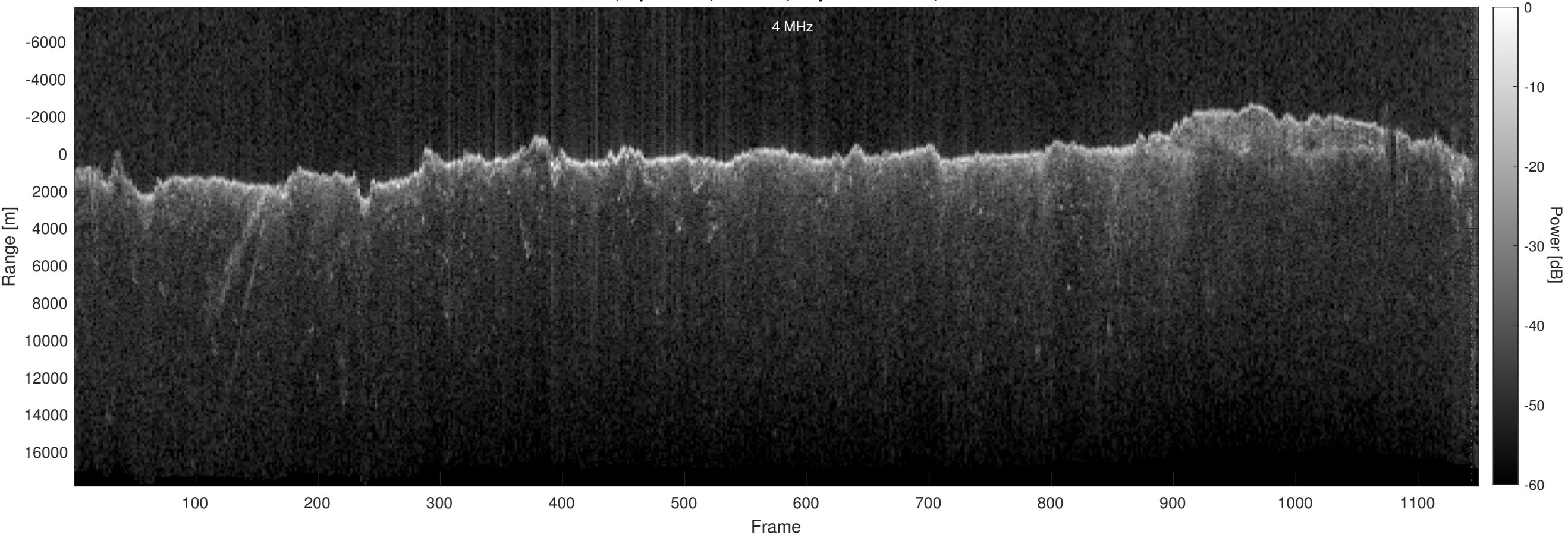
Orbit 13122, Optimized, Window, Depth-Corrected, Channel 2
