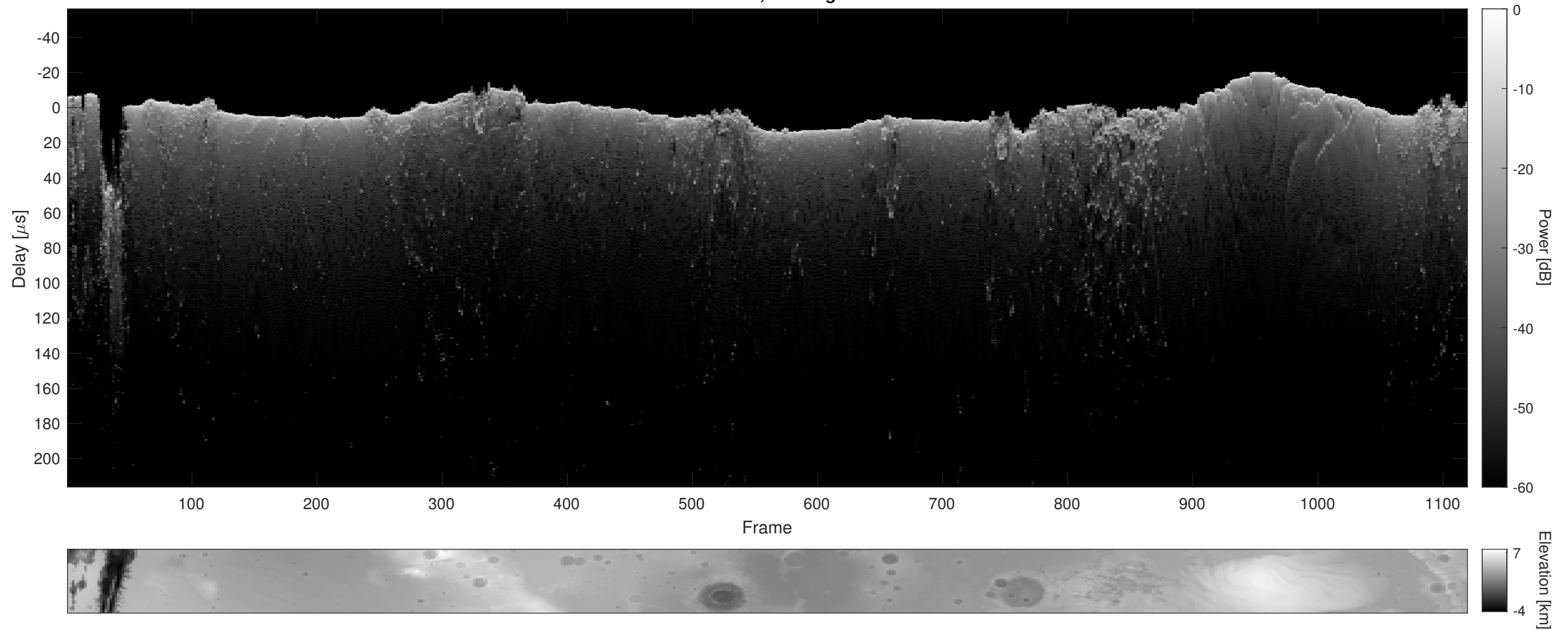
Orbit 13123, Cluttergram
