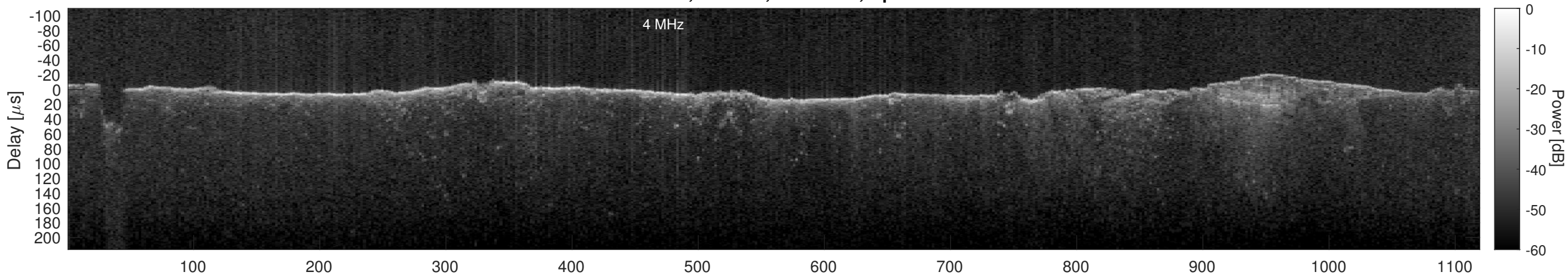
Orbit 13123, Cluttergram
