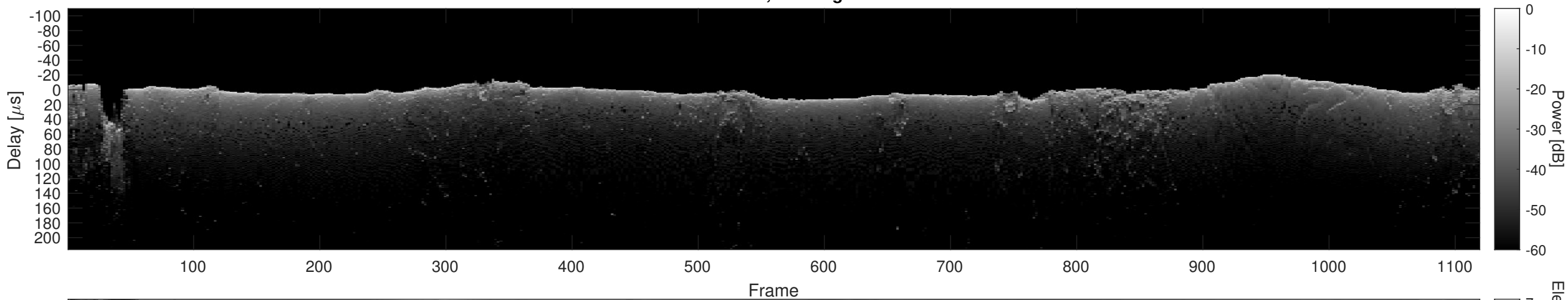
Orbit 13123, Cluttergram
