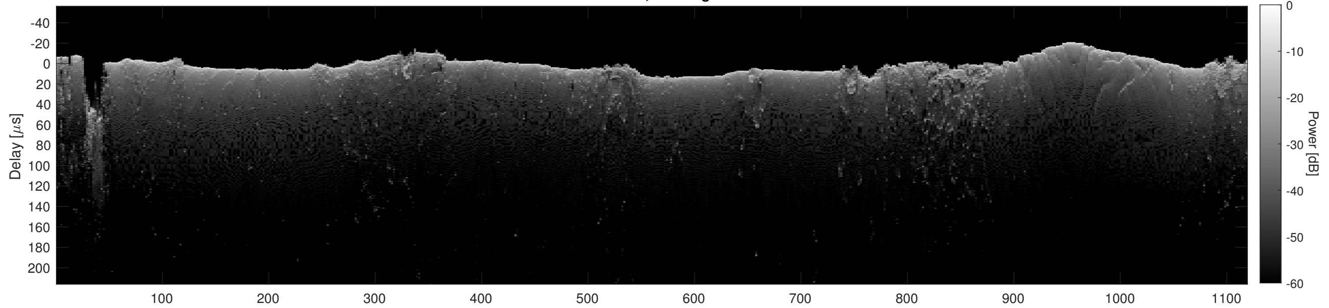
Orbit 13123, Cluttergram
