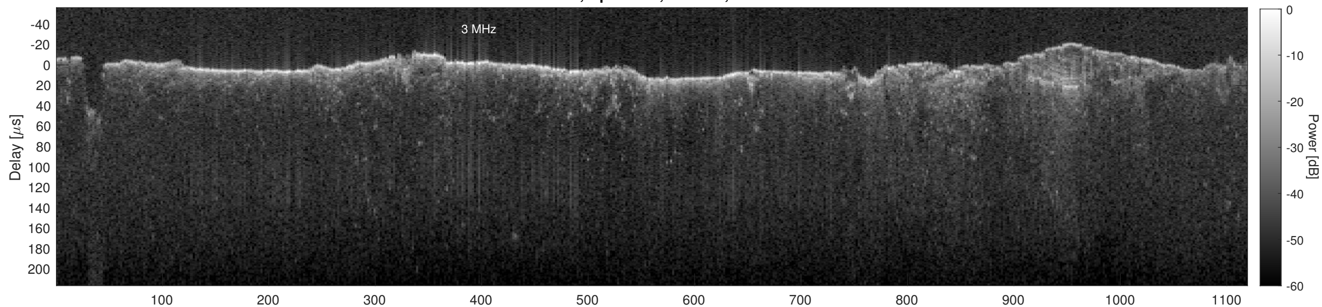
Orbit 13123, Cluttergram
