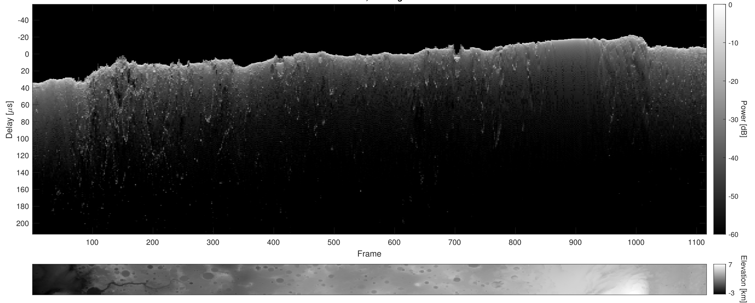
Orbit 13124, Cluttergram
