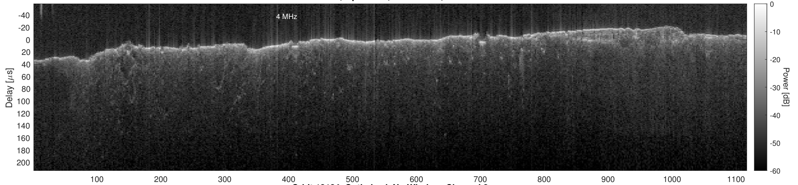
Orbit 13124, Optimized, No Window, Channel 2
