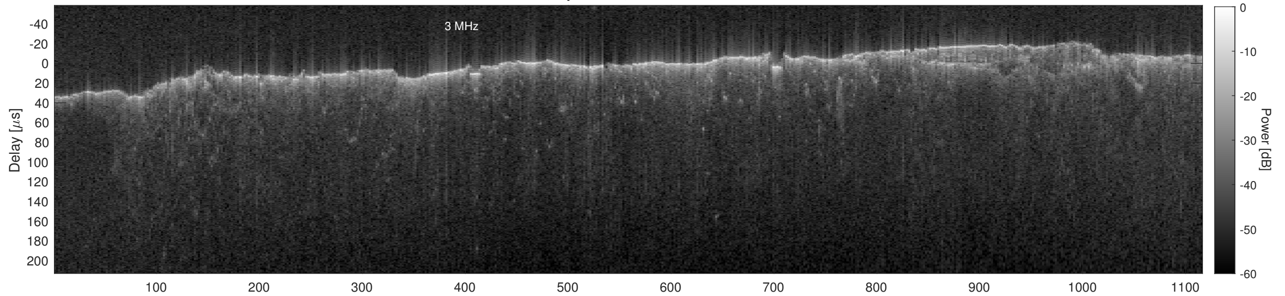
Orbit 13124, Cluttergram
