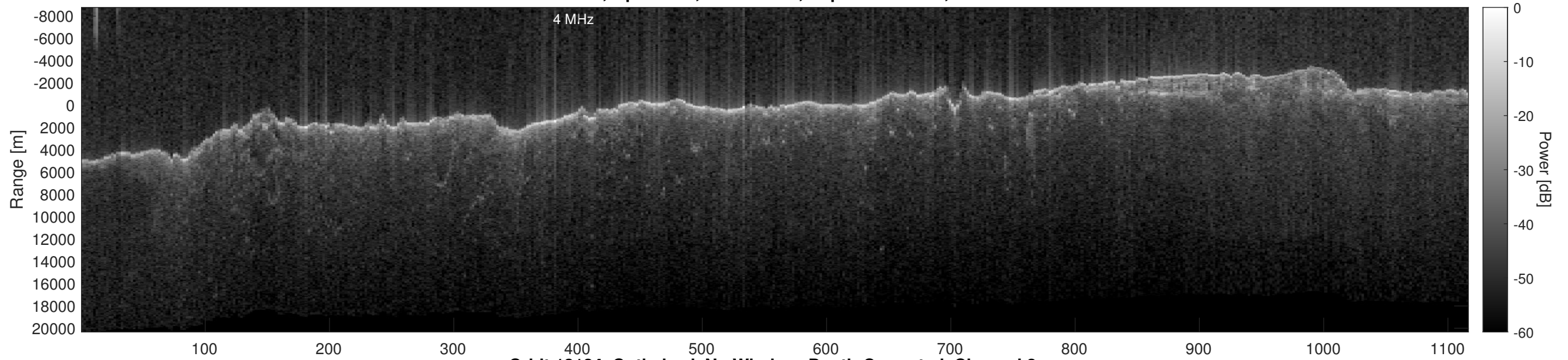
Orbit 13124, Optimized, No Window, Depth-Corrected, Channel 2
