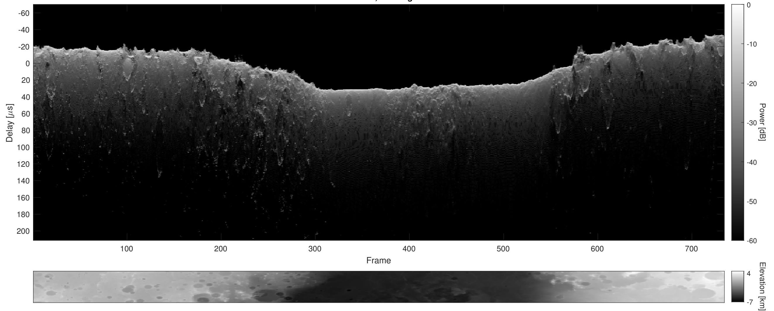
Orbit 13125, Cluttergram
