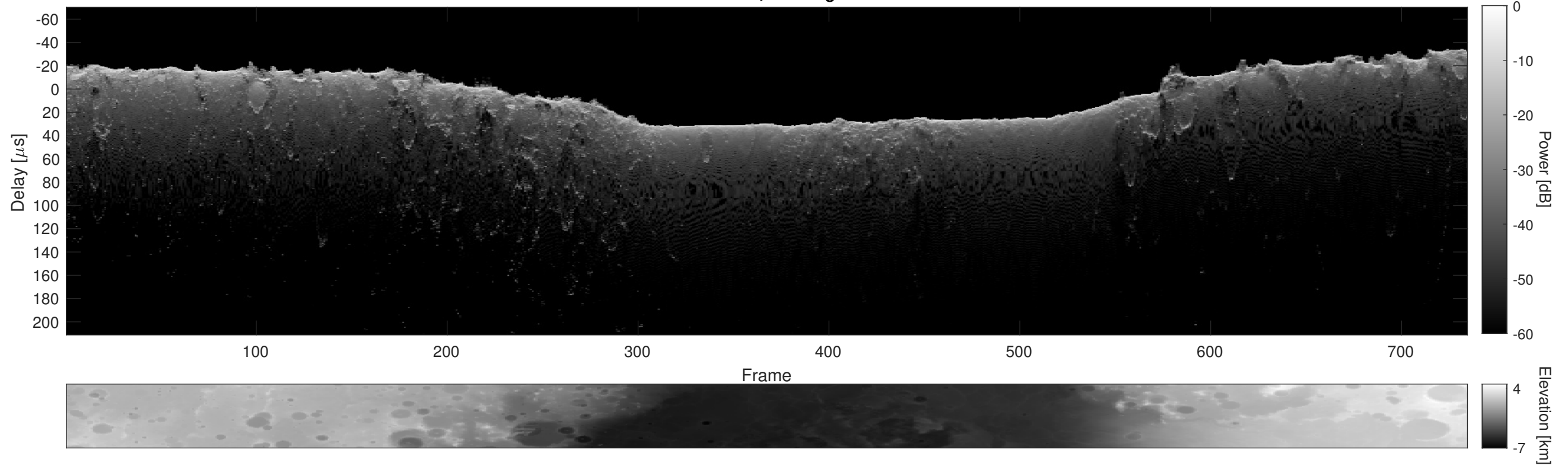
Orbit 13125, Cluttergram
