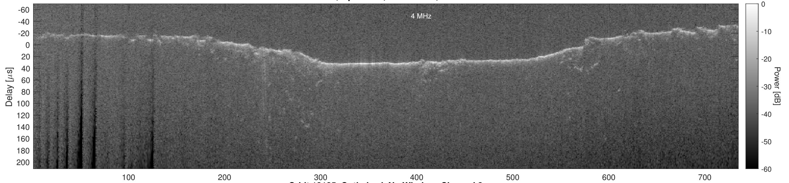
Orbit 13125, Optimized, No Window, Channel 2
