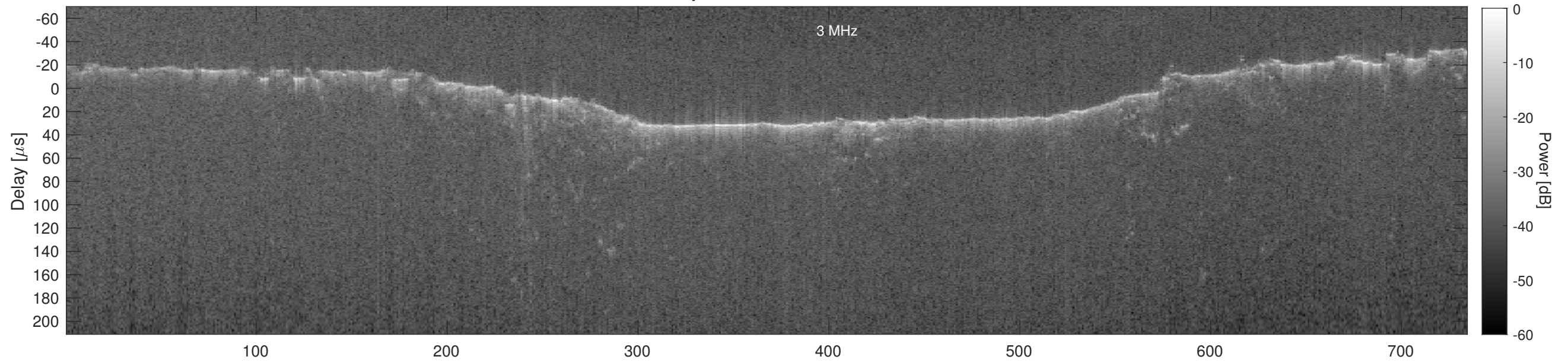
Orbit 13125, Cluttergram
