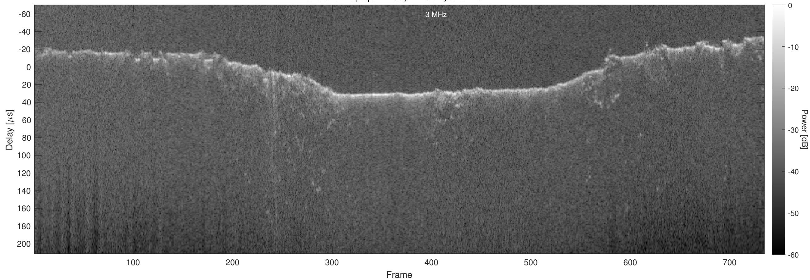
Orbit 13125, Optimized, Window, Channel 2
