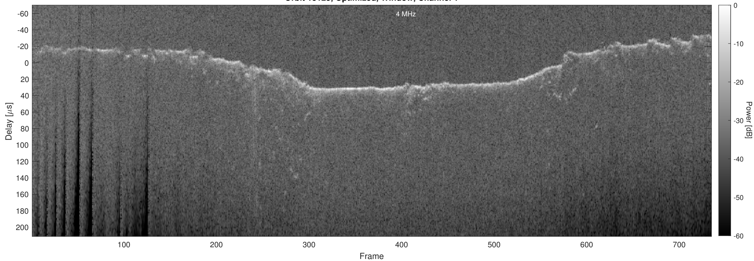
Orbit 13125, Optimized, Window, Channel 2
