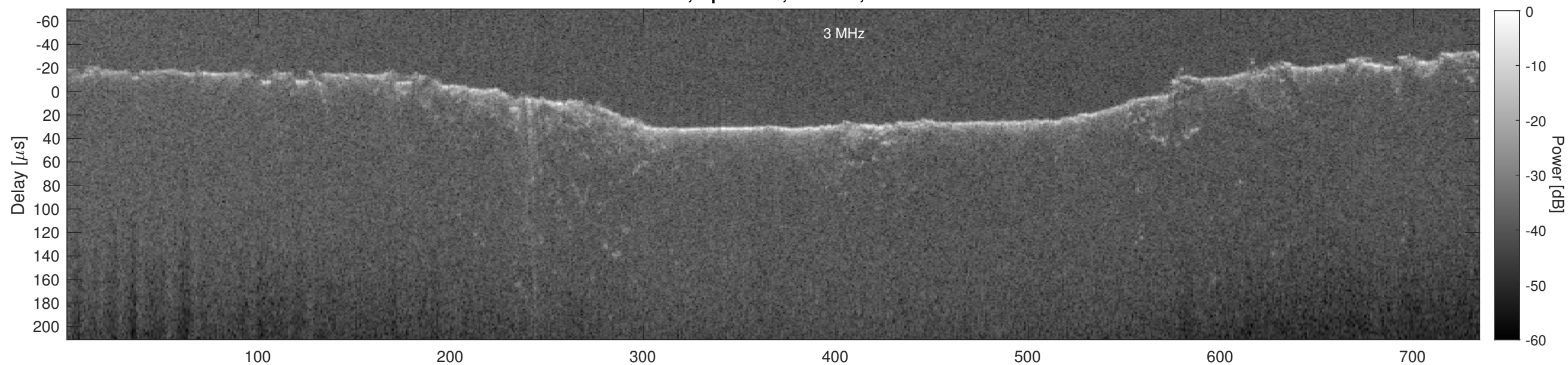
Orbit 13125, Cluttergram
