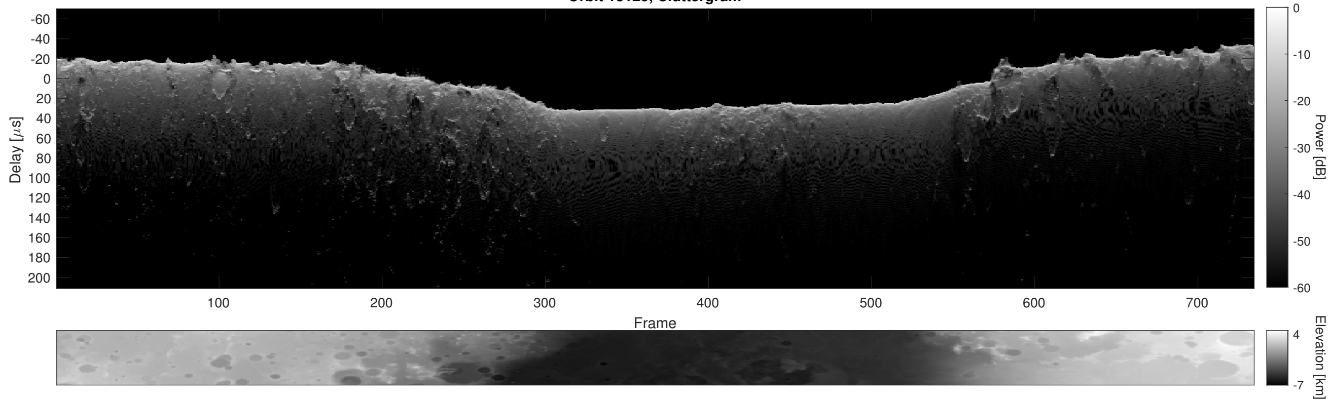
Orbit 13125, Cluttergram
