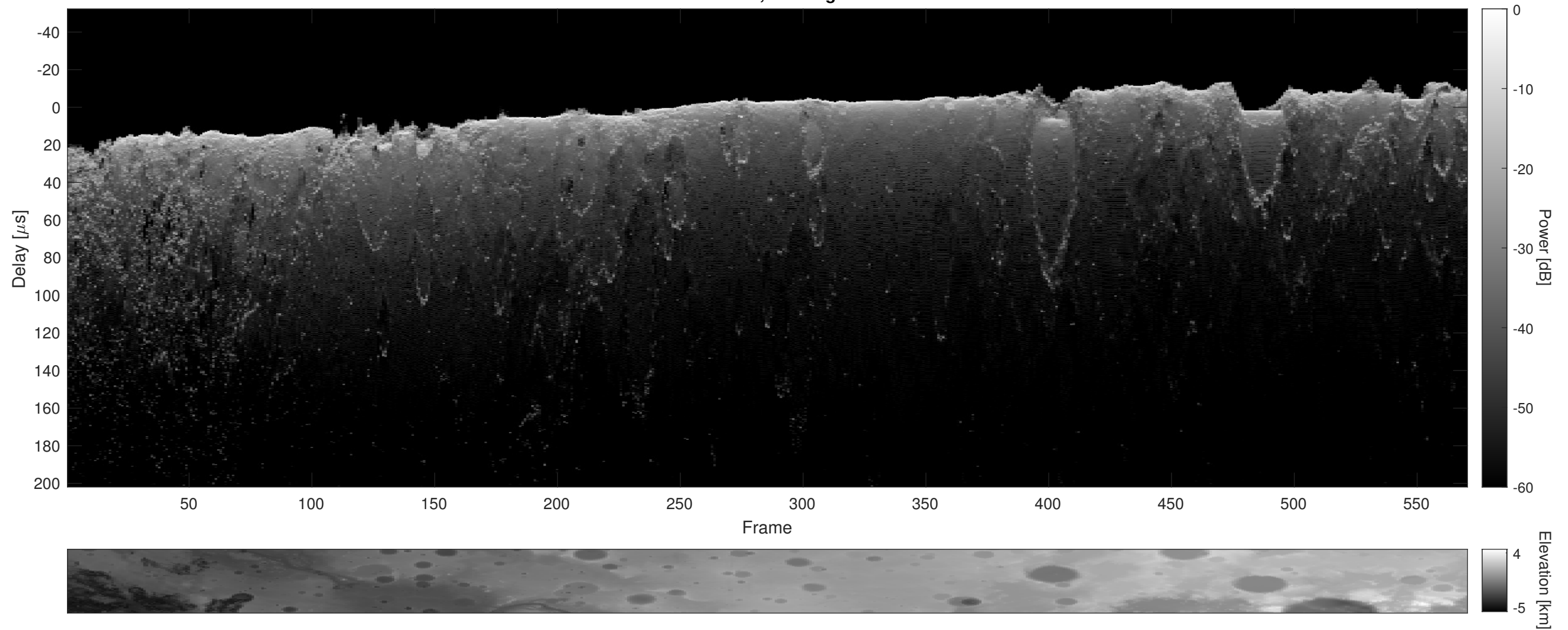
Orbit 13126, Cluttergram
