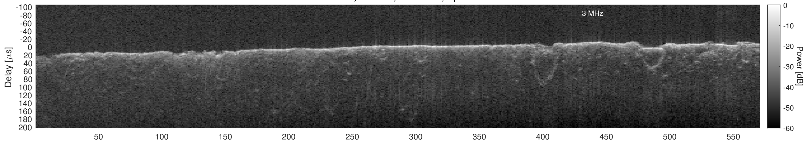
Orbit 13126, Cluttergram
