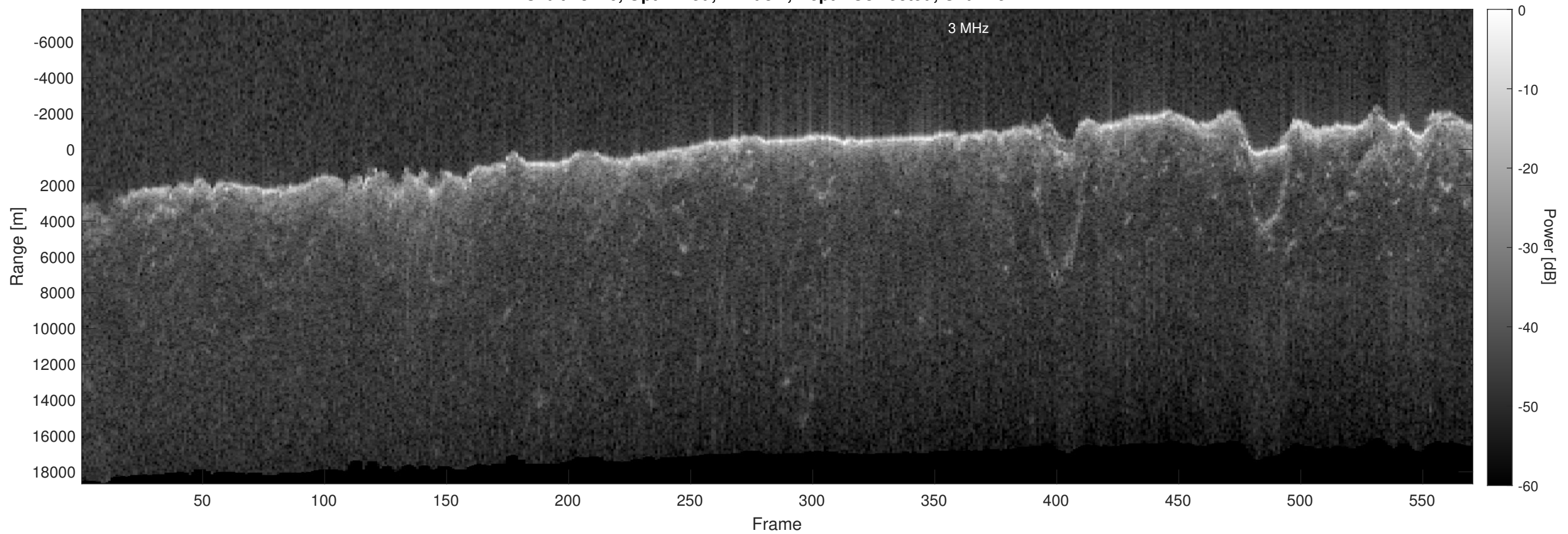
Orbit 13126, Optimized, Window, Depth-Corrected, Channel 2
