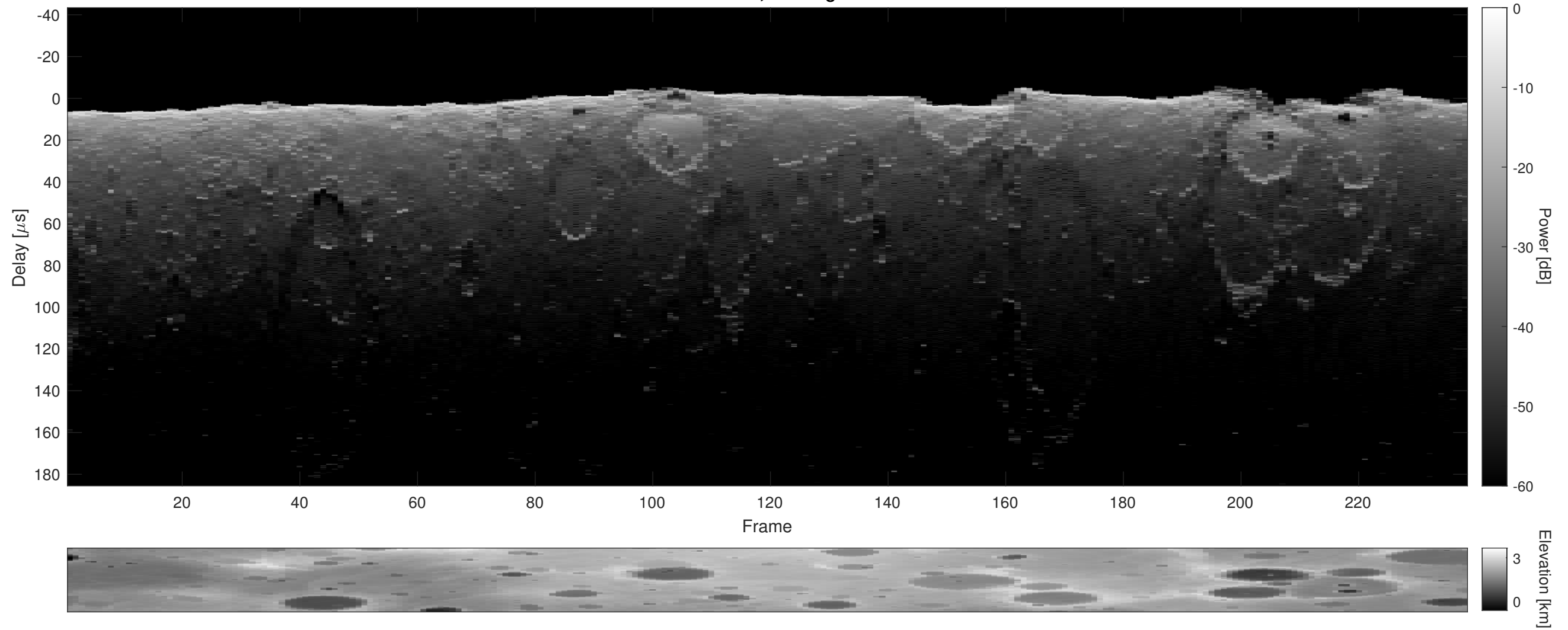
Orbit 13129, Cluttergram
