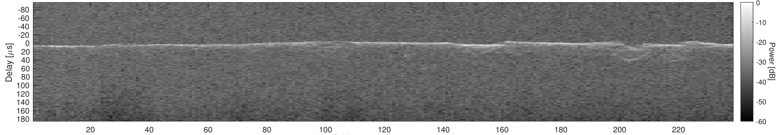
Orbit 13129, Cluttergram
