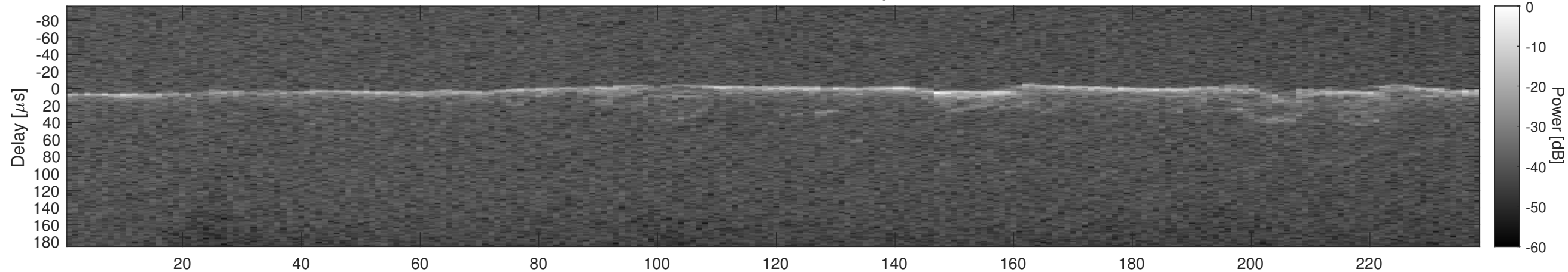
Orbit 13129, Cluttergram
