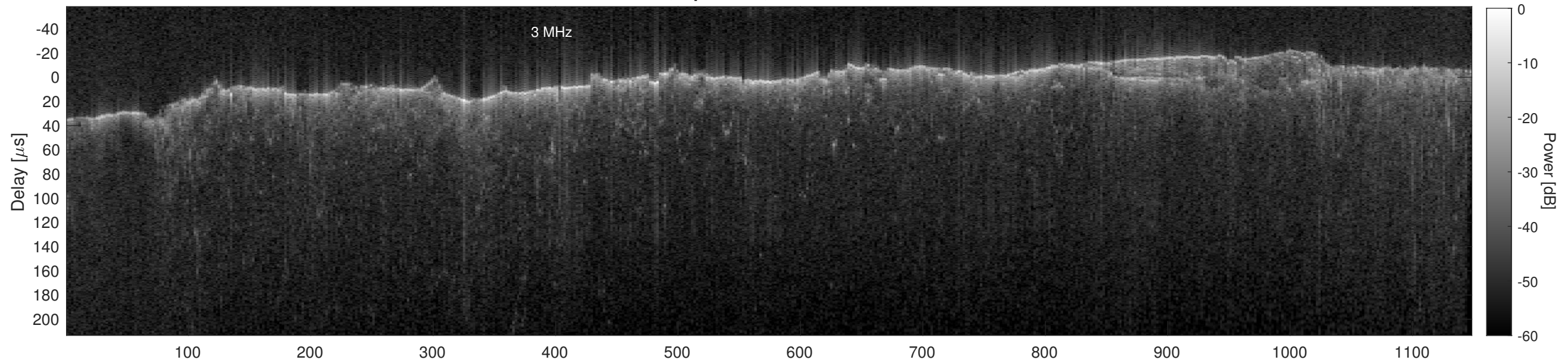
Orbit 13131, Cluttergram
