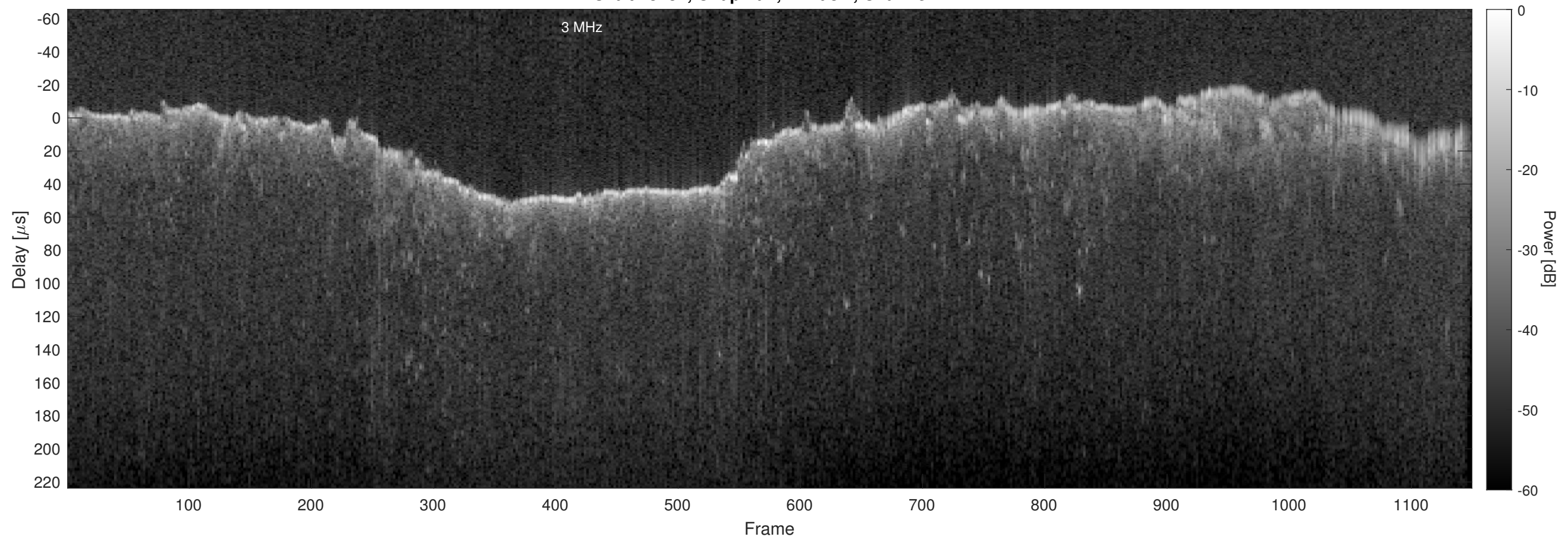
Orbit 13132, Chapman, Window, Channel 2
