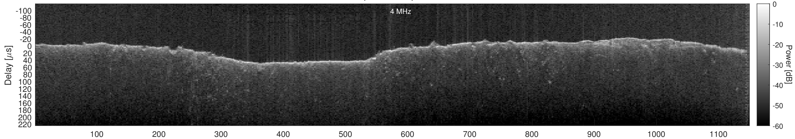
Orbit 13132, Window, Channel 1, Chapman
