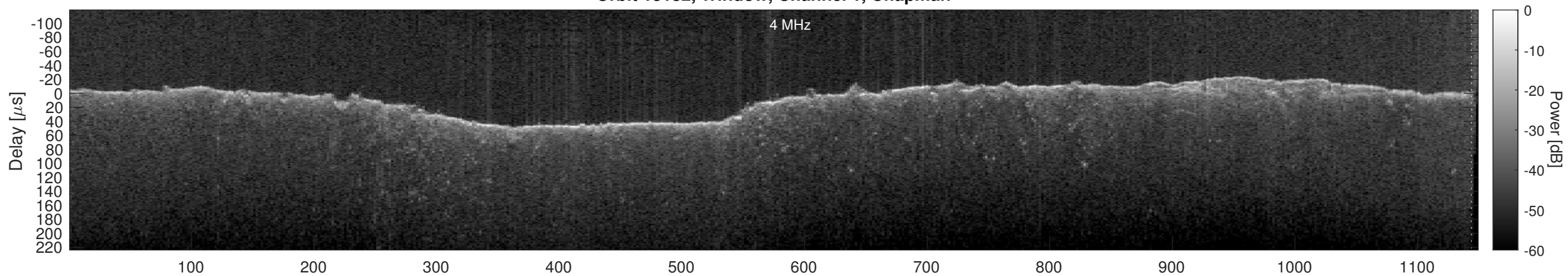
Orbit 13132, Window, Channel 1, Optimized
