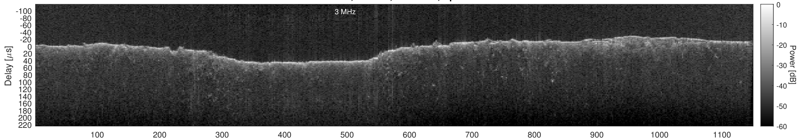
Orbit 13132, Cluttergram
