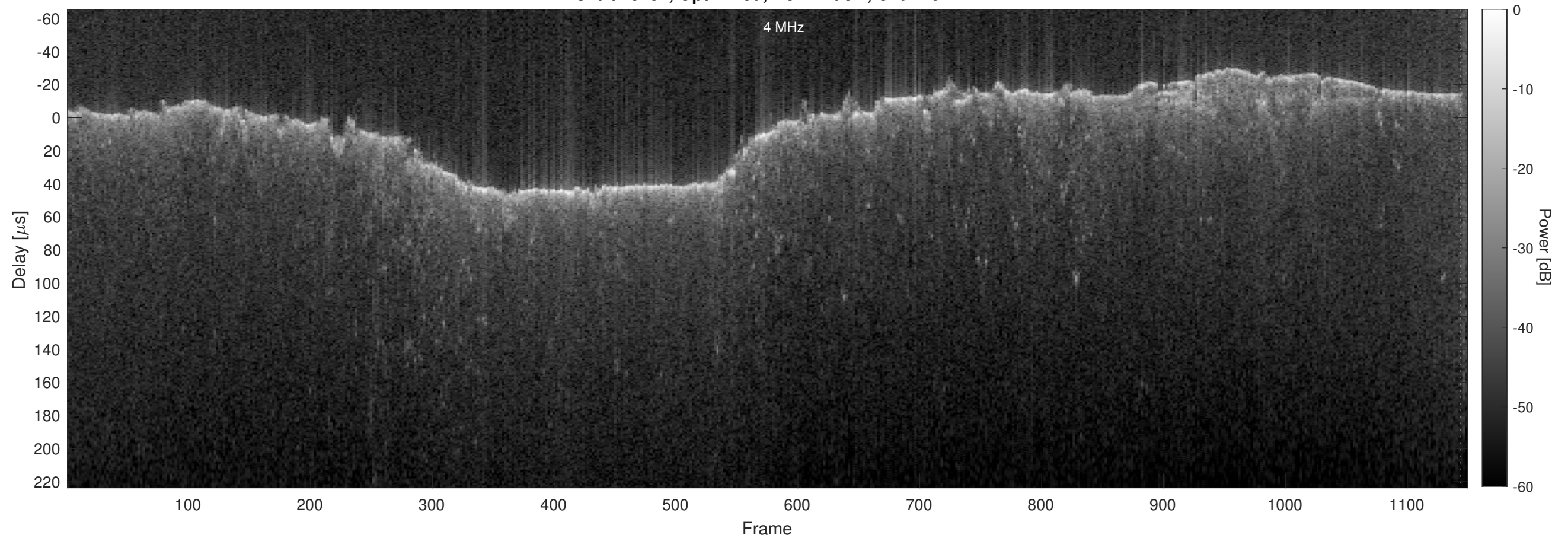
Orbit 13132, Optimized, No Window, Channel 2
