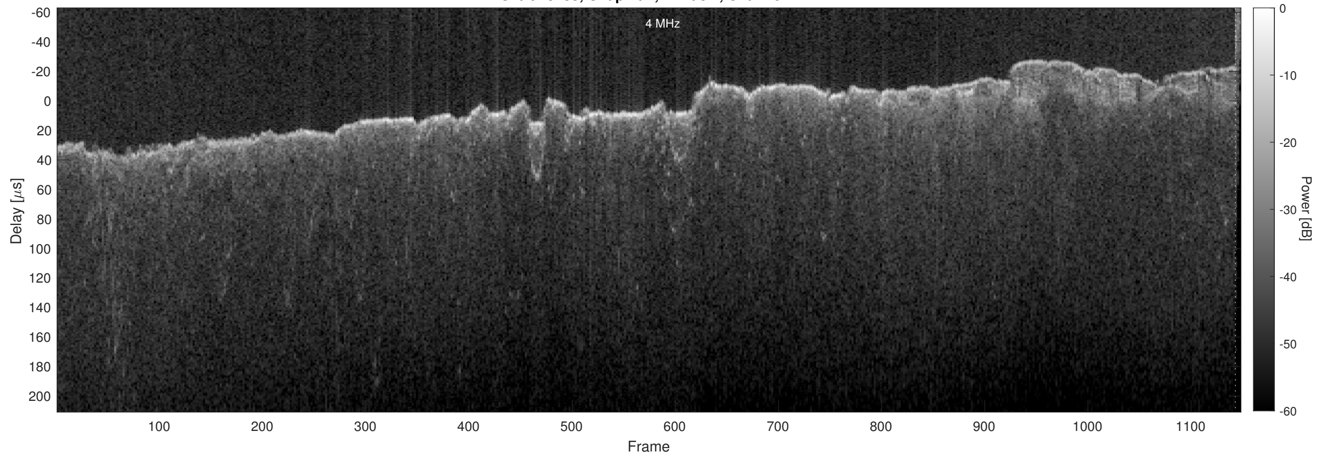
Orbit 13133, Chapman, Window, Channel 2
