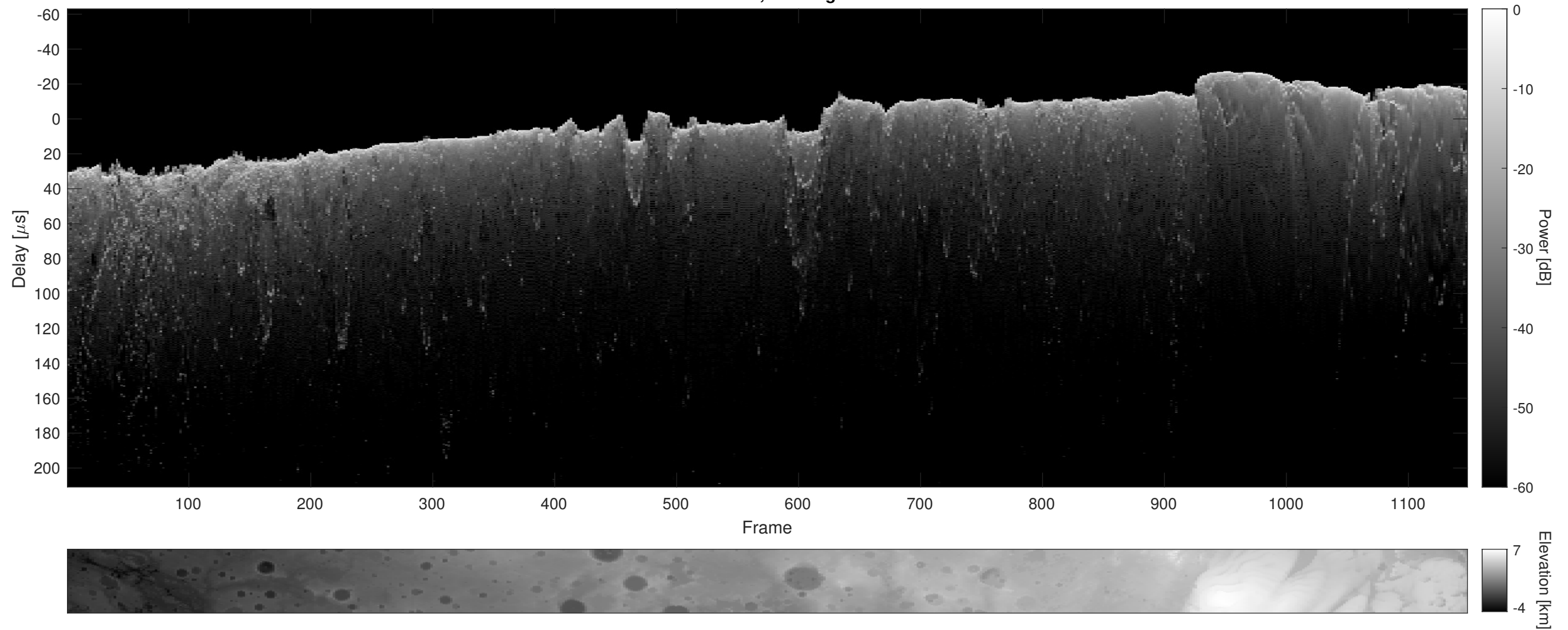
Orbit 13133, Cluttergram
