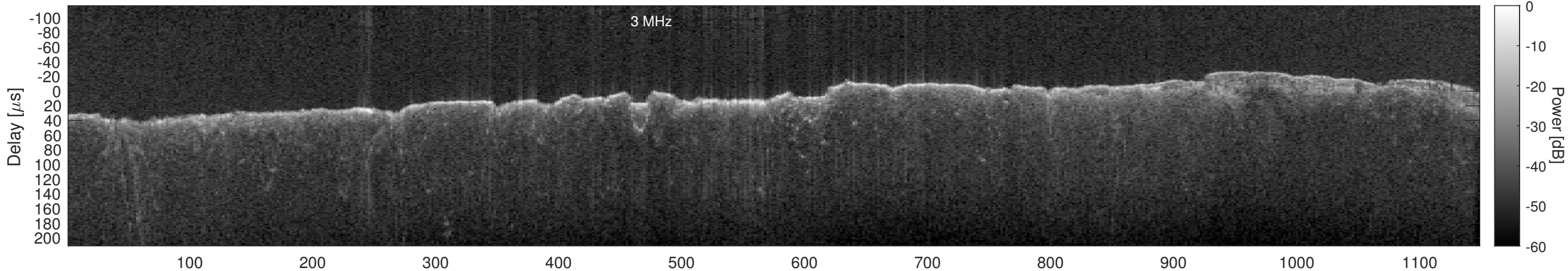
Orbit 13133, Window, Channel 2, Chapman
