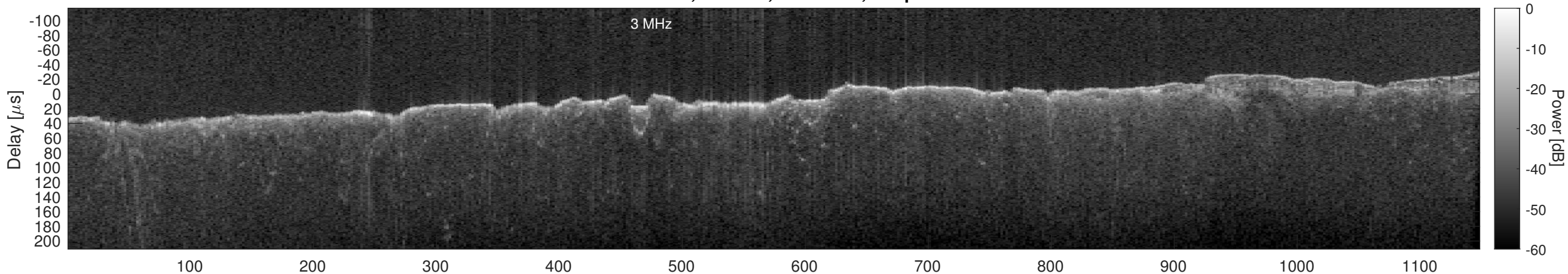
Orbit 13133, Window, Channel 2, Optimized
