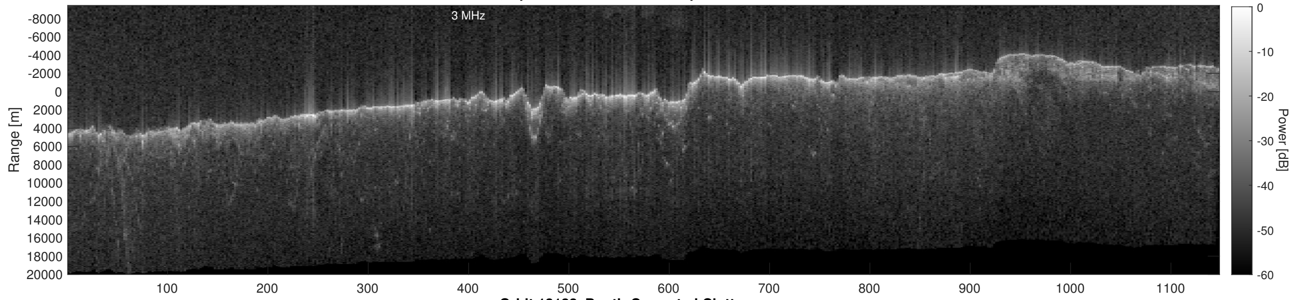
Orbit 13133, Depth-Corrected Cluttergram
