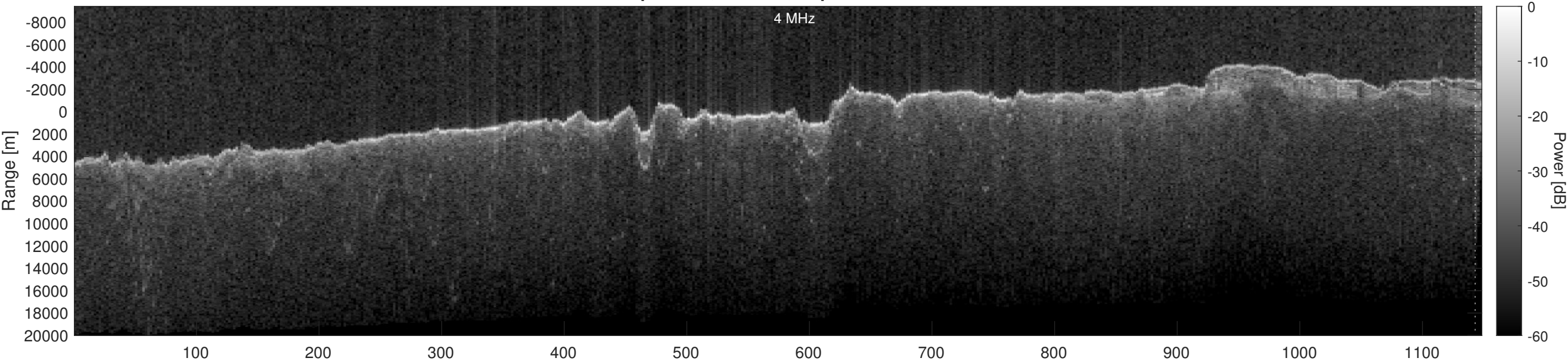
Orbit 13133, Optimized, Window, Depth-Corrected, Channel 2
