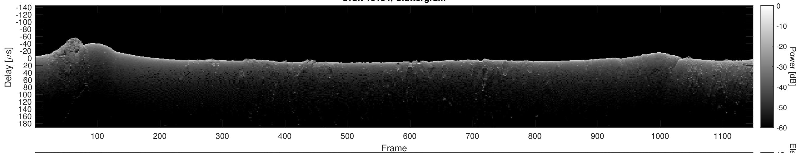
Orbit 13134, Cluttergram
