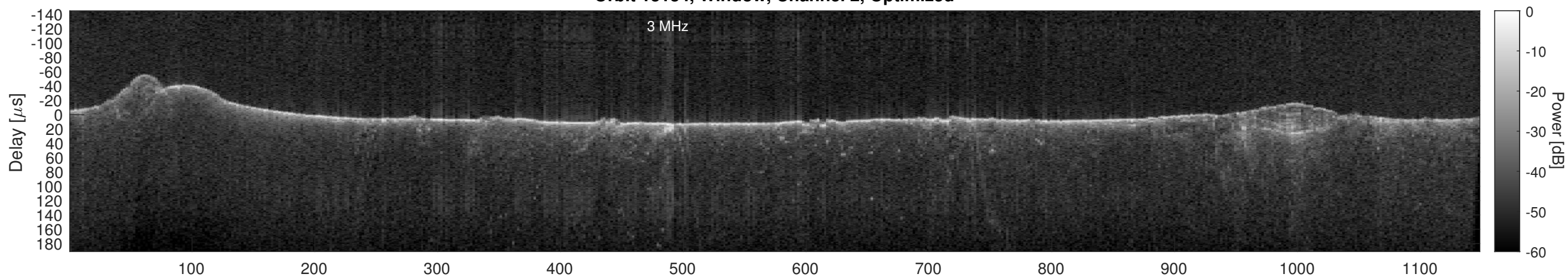
Orbit 13134, Cluttergram
