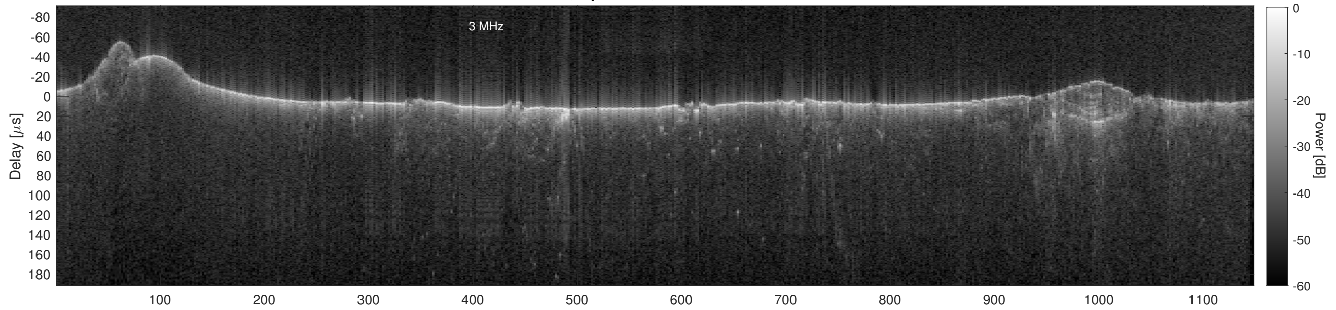
Orbit 13134, Cluttergram
