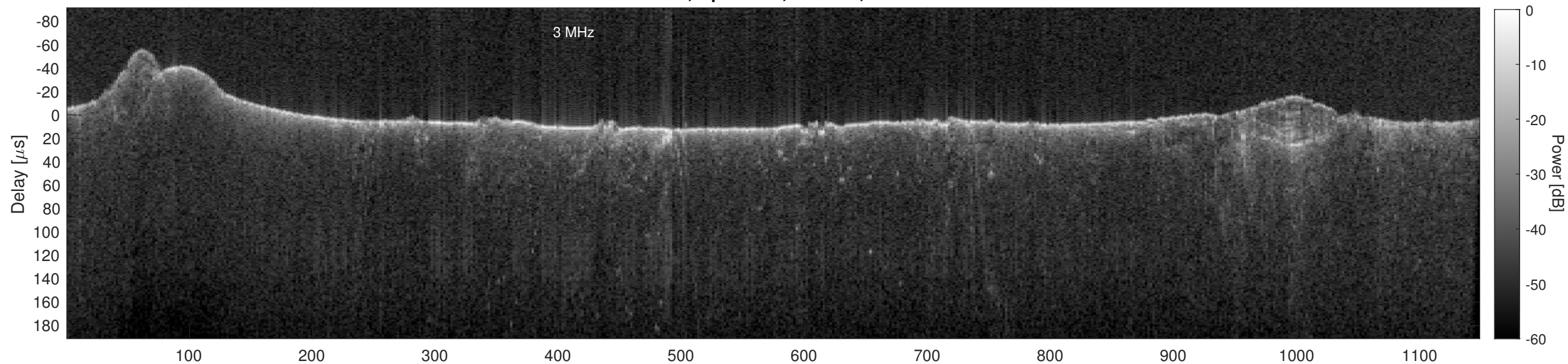
Orbit 13134, Cluttergram
