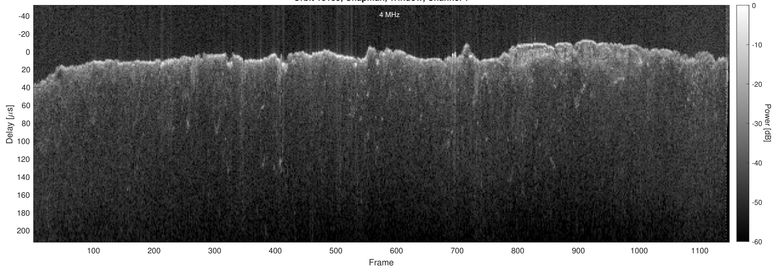
Orbit 13135, Chapman, Window, Channel 2
