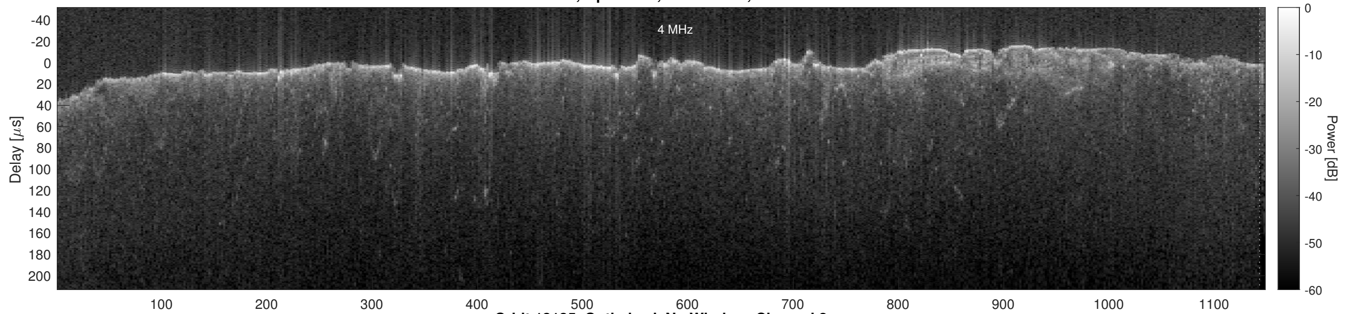
Orbit 13135, Optimized, No Window, Channel 2
