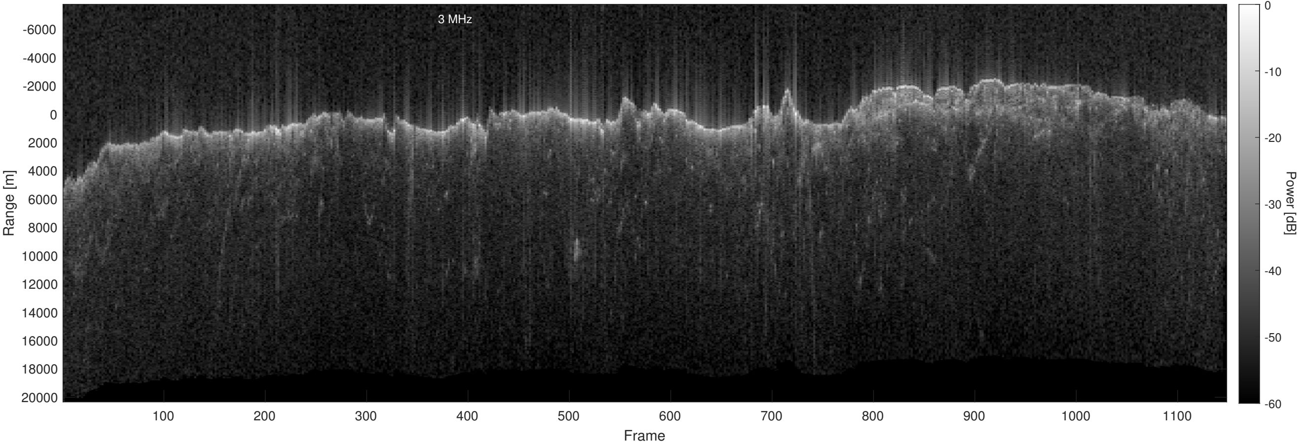
Orbit 13135, Optimized, No Window, Depth-Corrected, Channel 2
