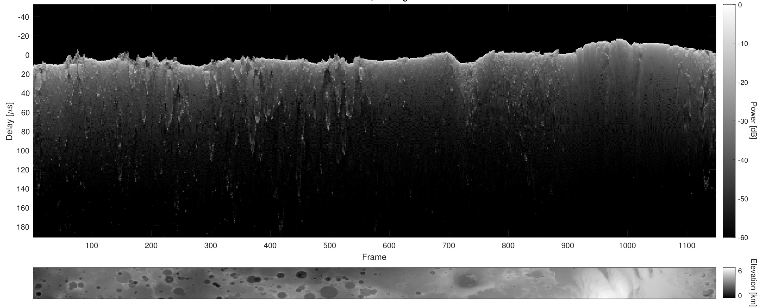
Orbit 13136, Cluttergram
