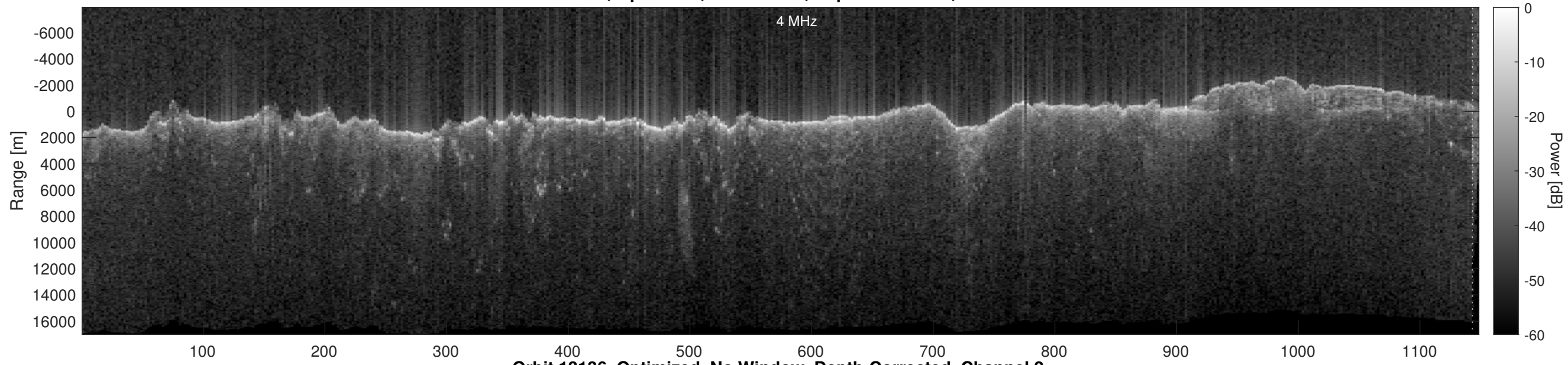
Orbit 13136, Optimized, No Window, Depth-Corrected, Channel 2
