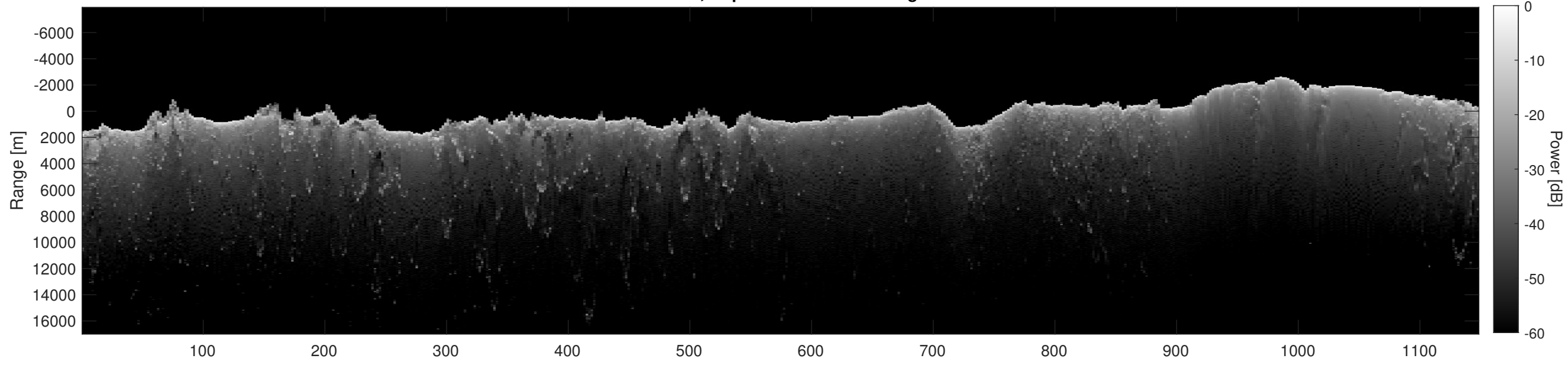
Orbit 13136, Depth-Corrected Cluttergram
