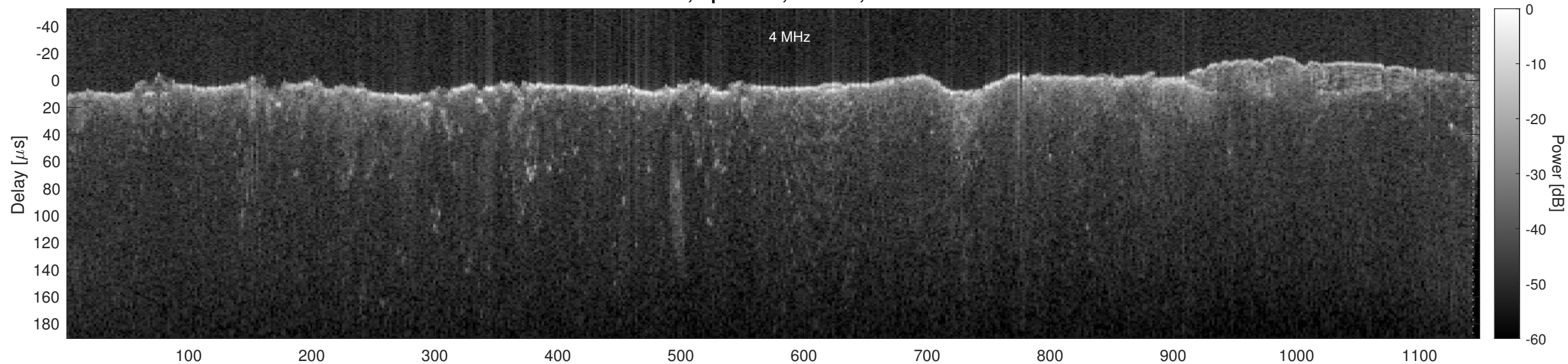
Orbit 13136, Optimized, Window, Channel 2
