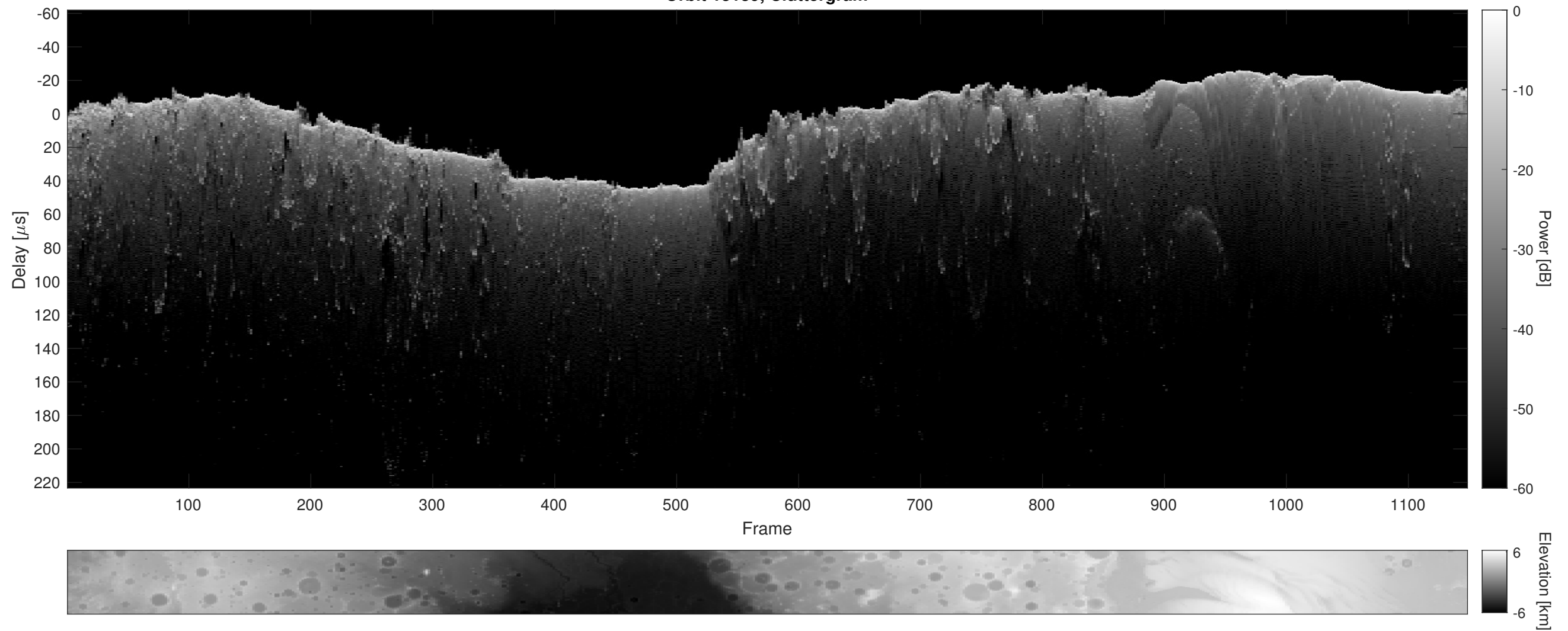
Orbit 13139, Cluttergram
