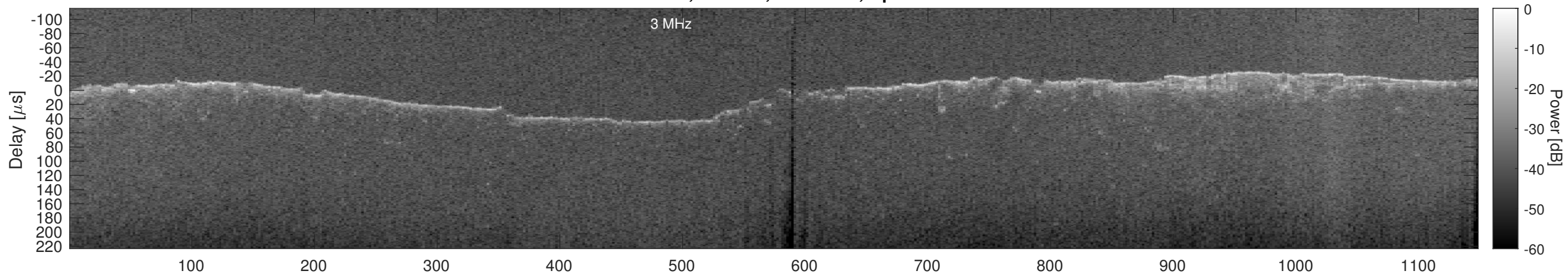
Orbit 13139, Cluttergram
