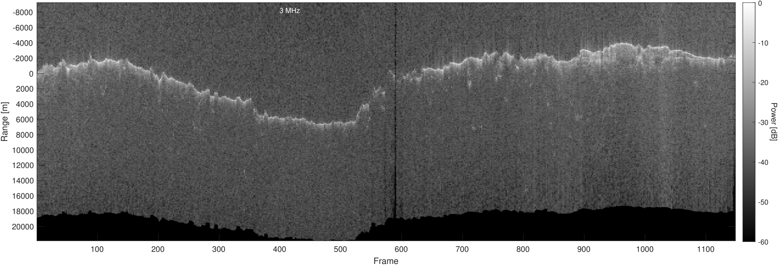
Orbit 13139, Optimized, No Window, Depth-Corrected, Channel 2
