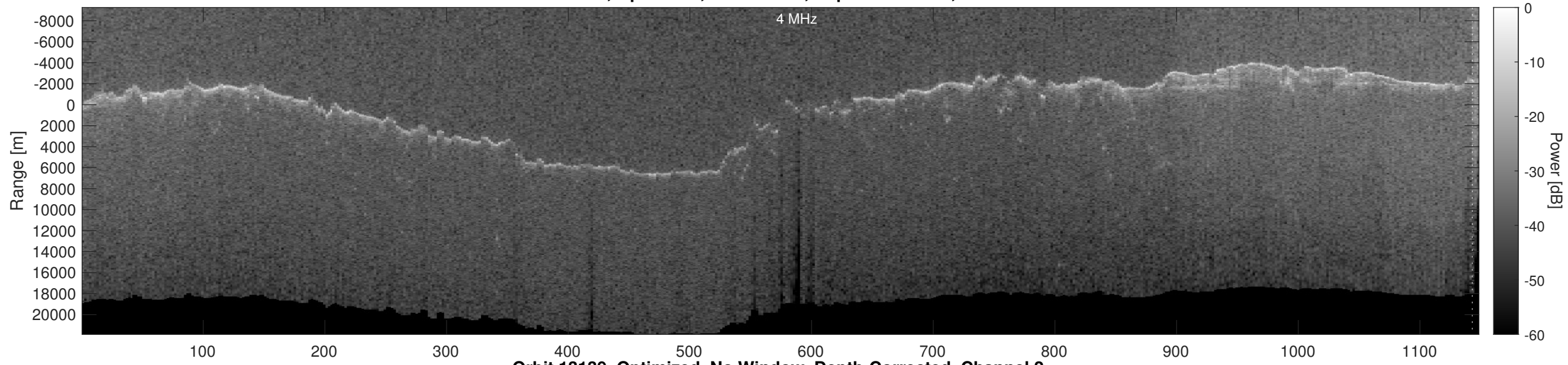
Orbit 13139, Optimized, No Window, Depth-Corrected, Channel 2
