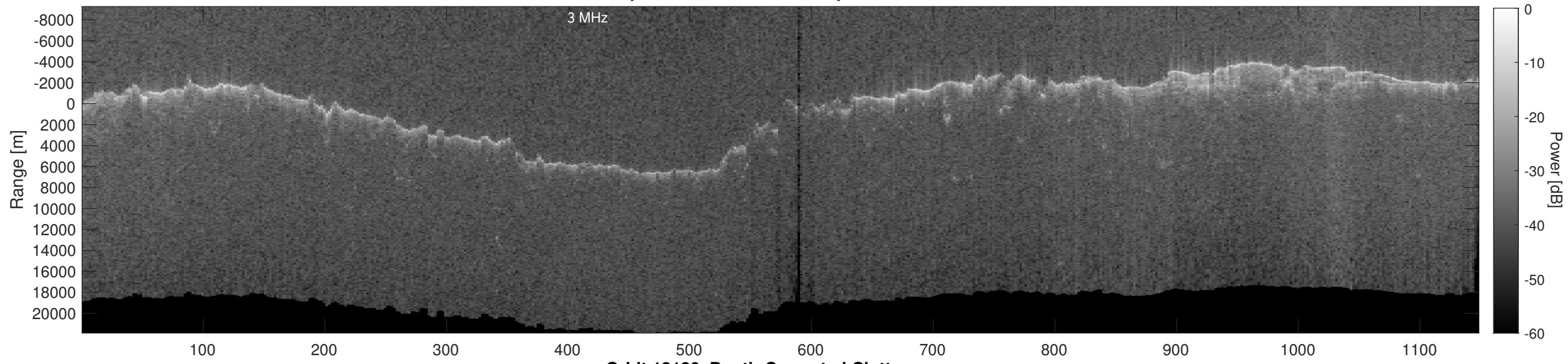
Orbit 13139, Depth-Corrected Cluttergram
