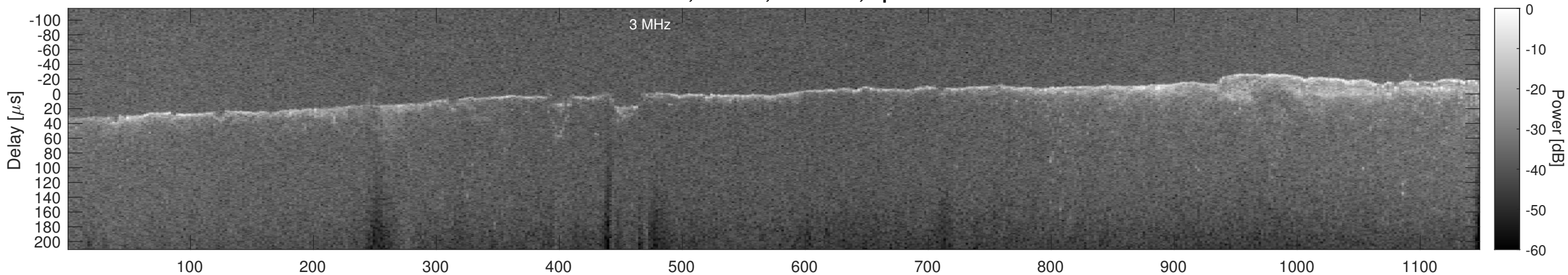
Orbit 13140, Cluttergram
