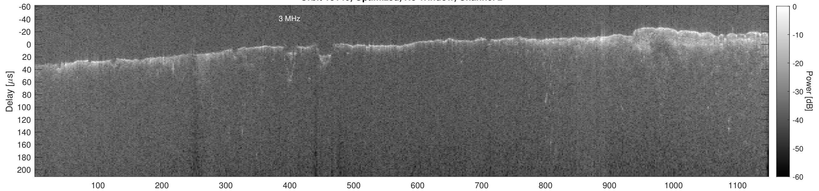
Orbit 13140, Cluttergram
