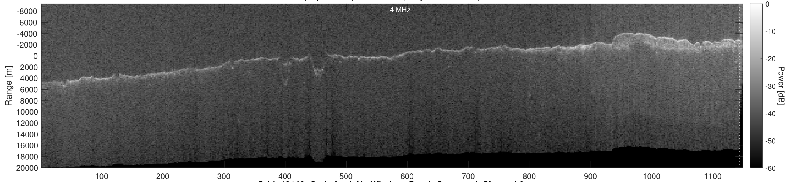
Orbit 13140, Optimized, No Window, Depth-Corrected, Channel 2
